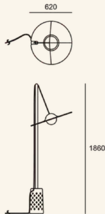
Schematic – dimensions in mm · manufacturer drawing
