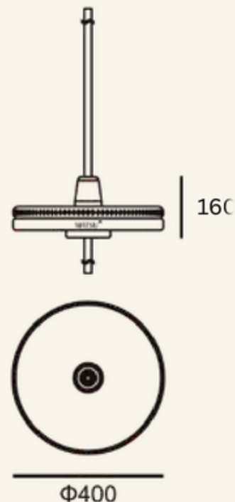
Schematic – dimensions in mm · manufacturer drawing
