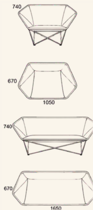
Schematic - dimensions in mm • manufacturer drawing
